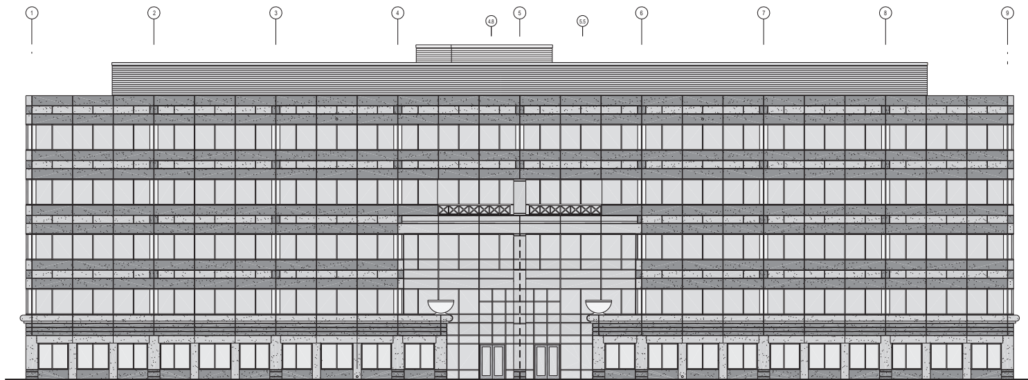
WEST & EAST ELEVATION
