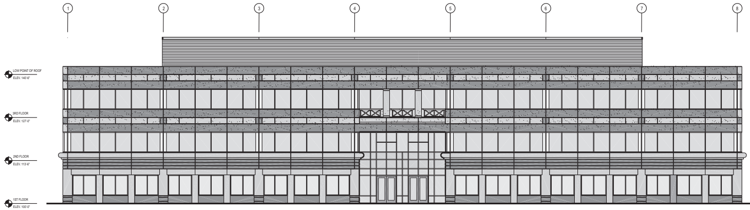
NORTH & SOUTH ELEVATION
