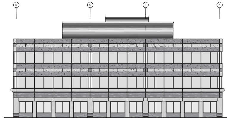
WEST ELEVATION
